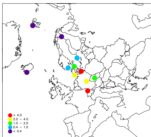
Figure 16: PCB-153 in air, 2009 ( \text{pg}/\text{m}^3 ).
