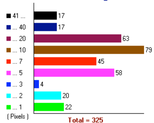
Pixel Histogram
