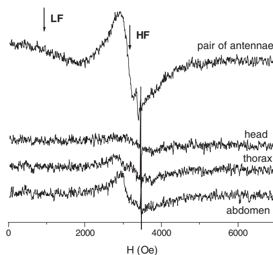
Figure 3. RT X-band ferromagnetic resonance spectra of S. quadripunctata body parts. Lines are guide to the eyes.
