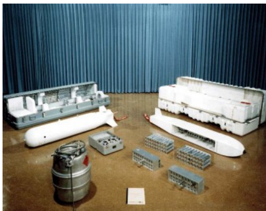
Fig. 10 – Photo of Cold Cloud Modification System
