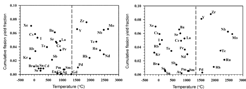
Figure 2. Cumulative yield fraction of ^{238}\text{U} and ^{235}\text{U} fast neutron fission product elements plotted vs ambient pressure melting point of each respective element. Dashed vertical line represents ambient pressure melting temperature of nickel silicide.
